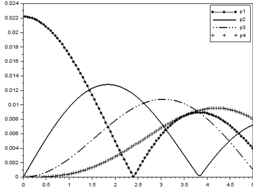
1) \{\mathbf{p}_1, \mathbf{p}_2, \mathbf{p}_3, \mathbf{p}_4\}, t = 0
