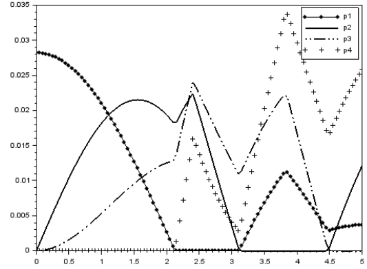
2) \{\mathbf{p}_1^\infty, \mathbf{p}_2^\infty, \mathbf{p}_3^\infty, \mathbf{p}_4^\infty\}, \alpha = -1
