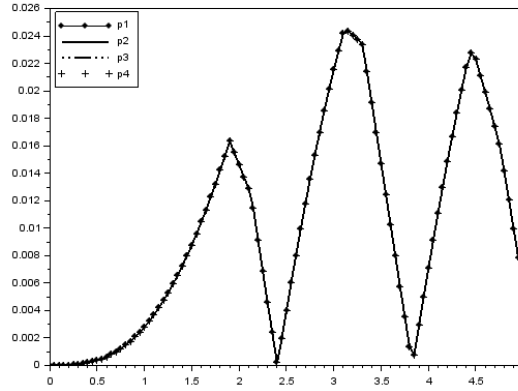
3) \{\mathbf{p}_1^\infty, \mathbf{p}_2^\infty, \mathbf{p}_3^\infty, \mathbf{p}_4^\infty\}, \alpha = 1
